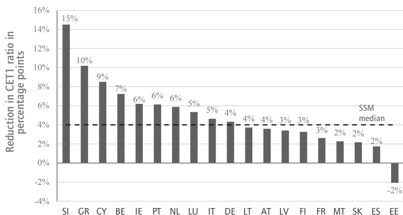
Figure 2.1: Comprehensive assessment impact on CET1 ratio under the adverse scenario
